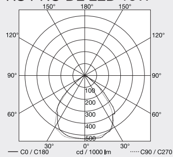
RS PRO DL LED 15W
